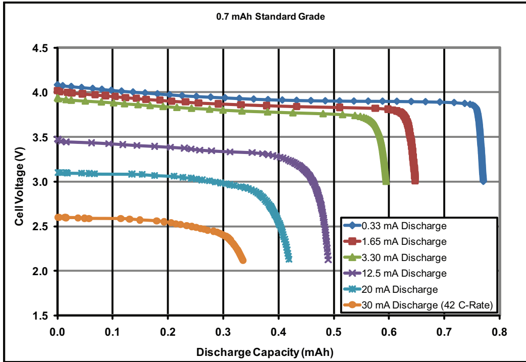
Figure 1: Typical Discharge Curves @25°C (0.7 mAh Standard Grade Cell)
