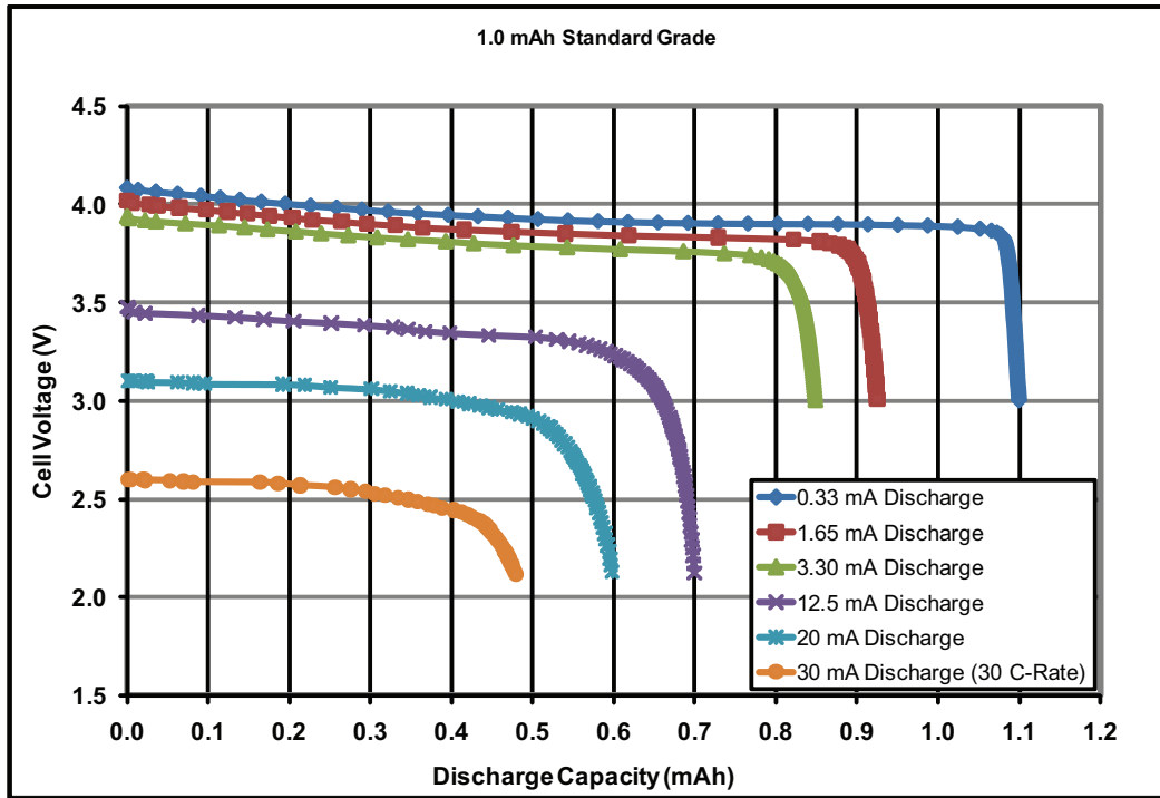
Figure 3: Typical Discharge Curves @25°C (1.0 mAh Standard Grade Cell)
