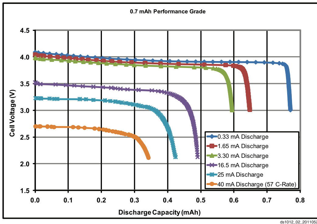
Figure 2: Typical Discharge Curves @25°C (0.7 mAh Performance Grade Cell)
