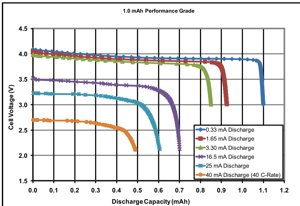
Figure 4: Typical Discharge Curves @25°C (1.0 mAh Performance Grade Cell)
